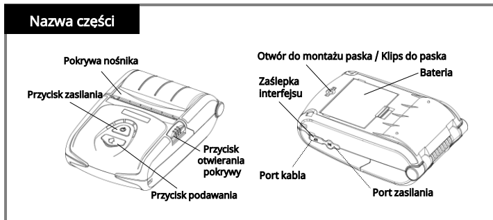
SPP-R200III
